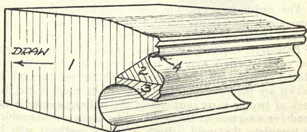
FIG. 55—SKETCH OF SPLIT PATTERN FOR STONE SHOWN IN FIG. 54
